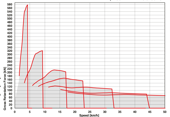
ADT, B60E 4X4 - Retardation
